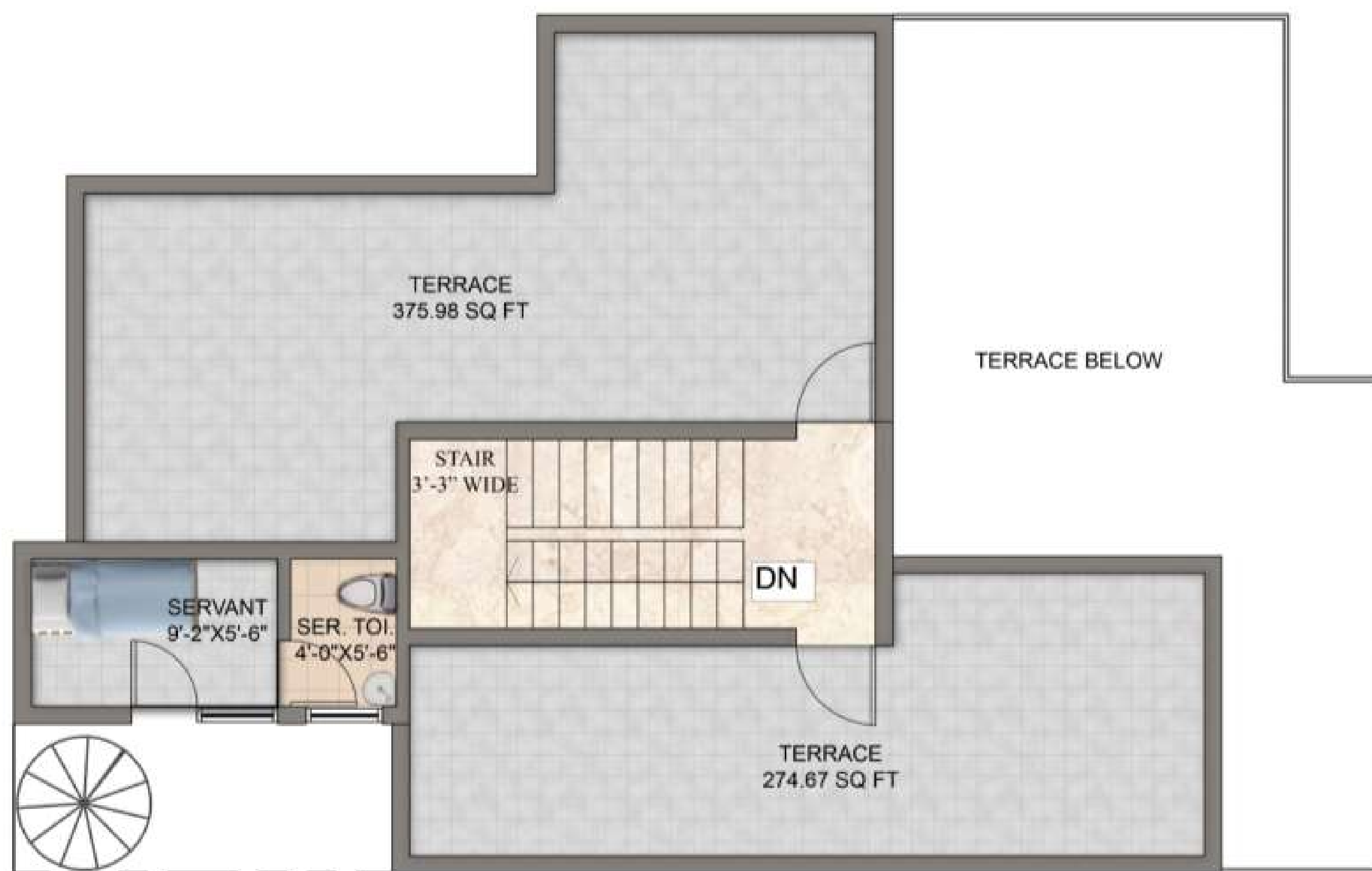
TERRACE PLAN
